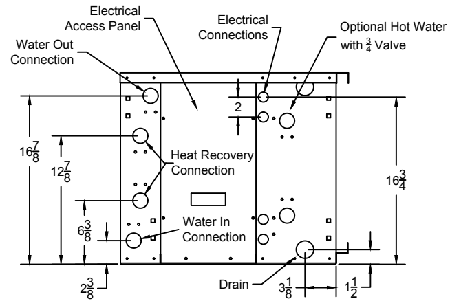
View "B"
