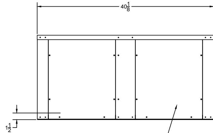
Elevation "B"
